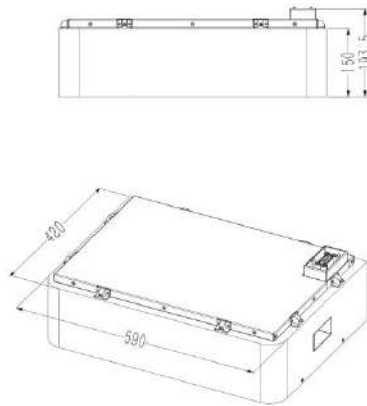
High voltage battery cluster control box
