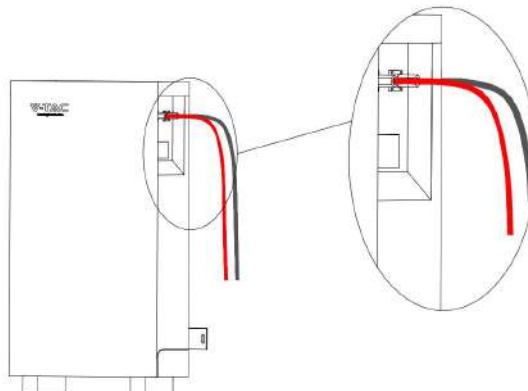
Fig.6-4 Power Cable Connection Diagram
