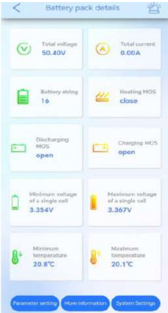
Figure 8: Battery pack details
