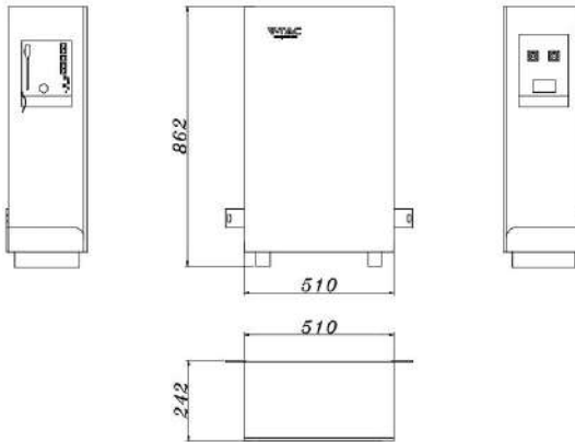
Fig. 5-1 Product Dimensions
